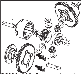
BS933-006 Centre diff. box
