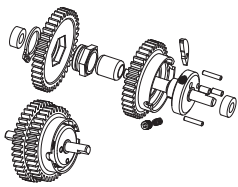
BS903-103 Gear-40T/37T
