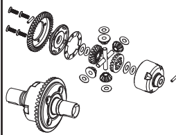
BS903-104 Diff. unit
